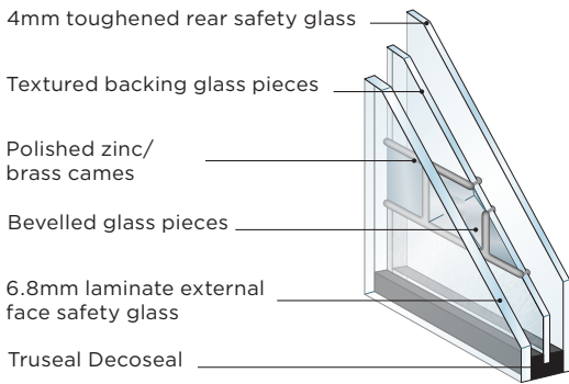
Diagram represents a typical make up of our triple glazed glass. Please contact us for further info
